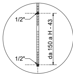
Detail of 2 lateral connections connection
